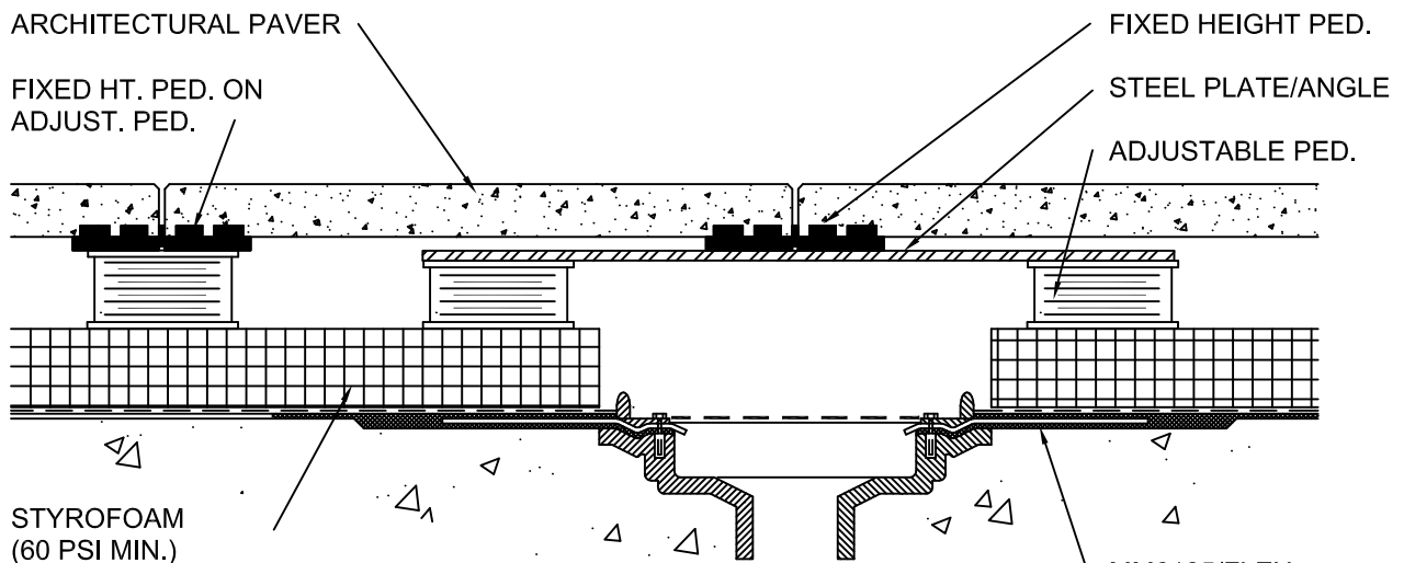
WHEN PAVER SUPPORTS LINE UP OVER DRAIN (ref. UA-5B for isometric layout)
