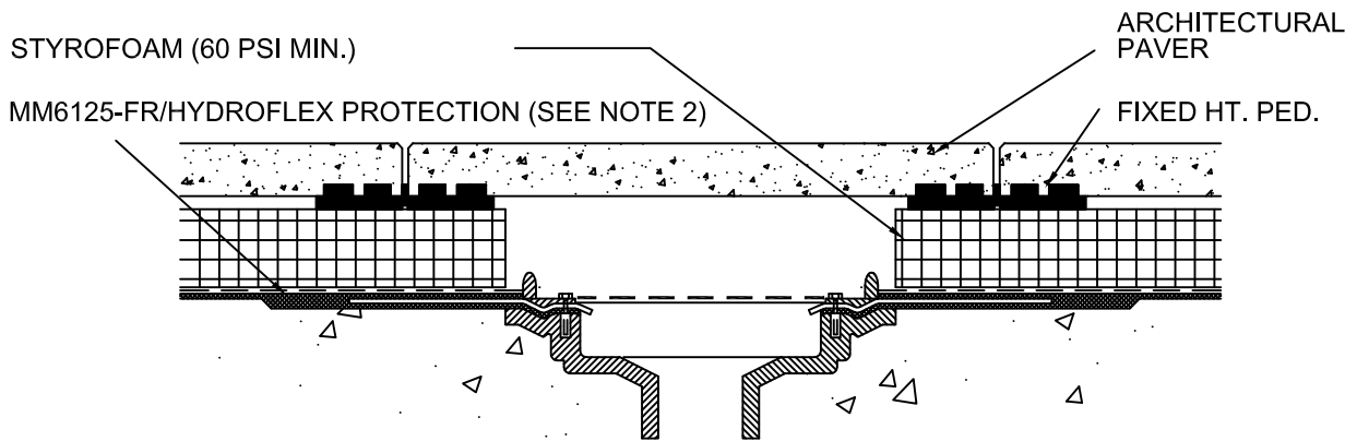
WHEN PAVER SUPPORTS CAN BE PLACED AROUND THE DRAIN
